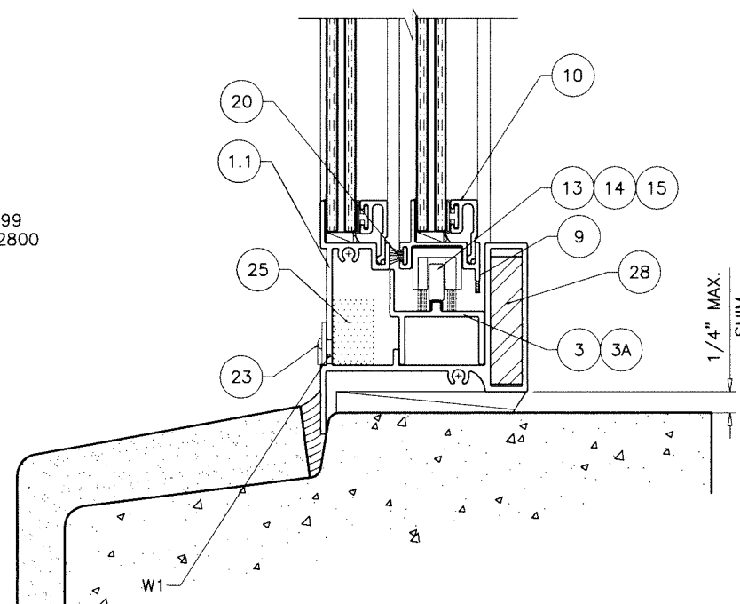
FRAME SILL TYPE '3' SILL WITHOUT ANCHORS SEE SHEET 6 FOR CAPACITY
