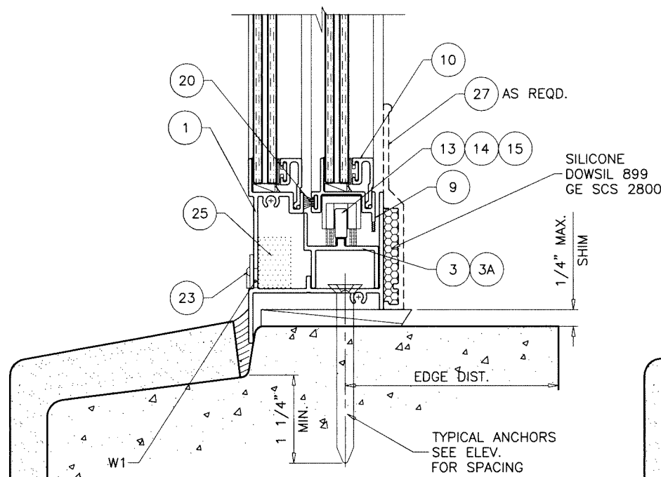
FRAME SILL TYPE '2' SILL WITH ANCHORS SEE SHEET 5 FOR CAPACITY
