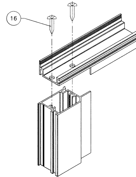
VENT TOP CORNER
