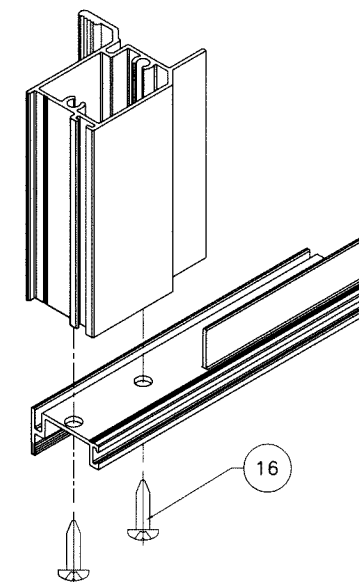
VENT BOTTOM CORNER
